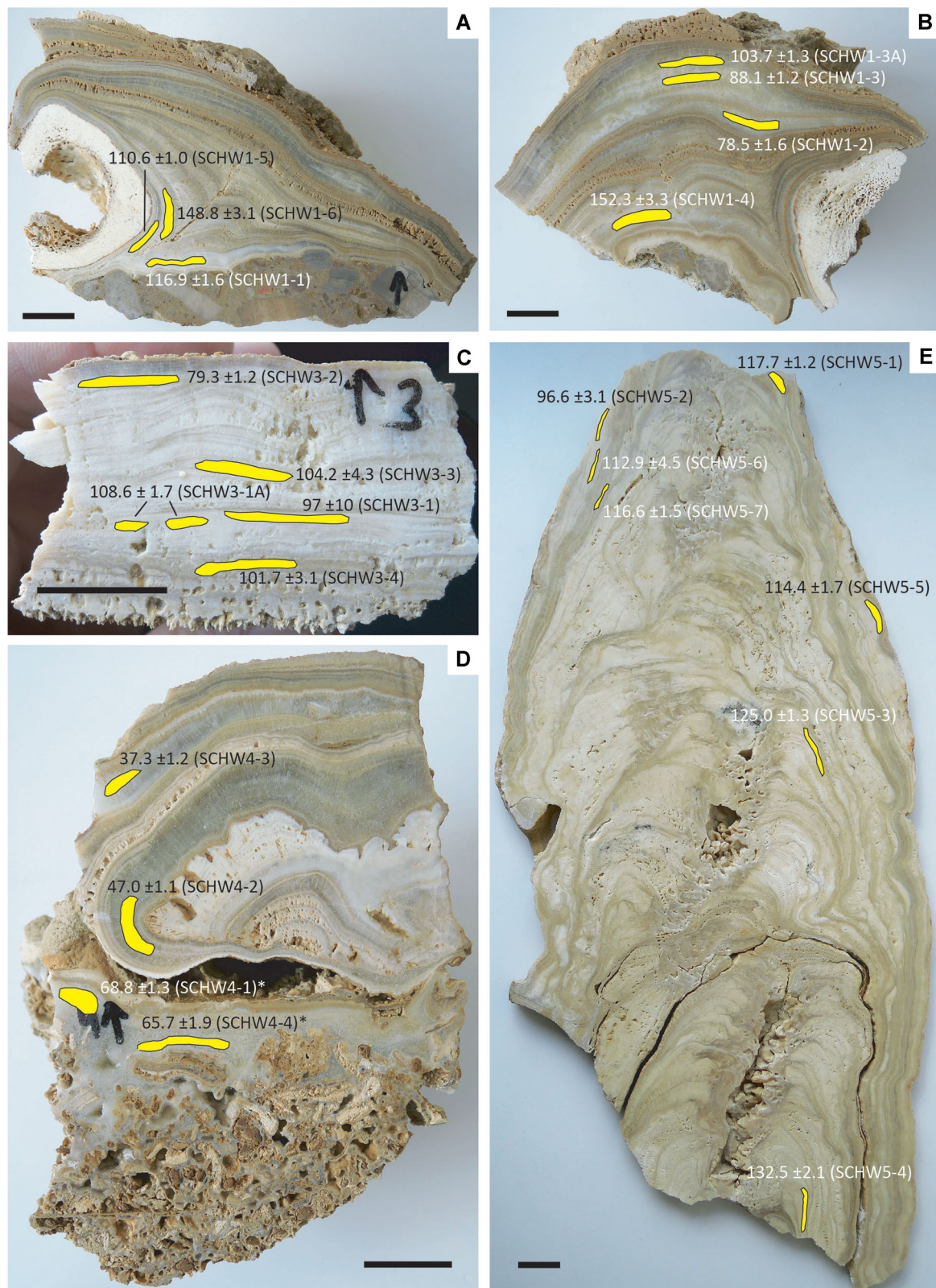
Figure 5. Slabbed speleothem specimens from Schwabenreith Cave showing ^{230}\text{Th}/\text{U} sampling spots (in yellow) and ages ( \text{ka} \pm 2\sigma errors). (A,B) Front and rear side of flowstone SCHW1 (ca. 2-cm-thick slab), which was deposited around a cave bear bone. (C) Sample SCHW3. (D) Sample SCHW4. Two subsamples were drilled from the backside and are marked by an asterisk (*). (E) Stalagmite SCHW5. Top is up on all samples, and scale bars are 2 cm in all images. [Color figure can be viewed at wileyonlinelibrary.com .]
